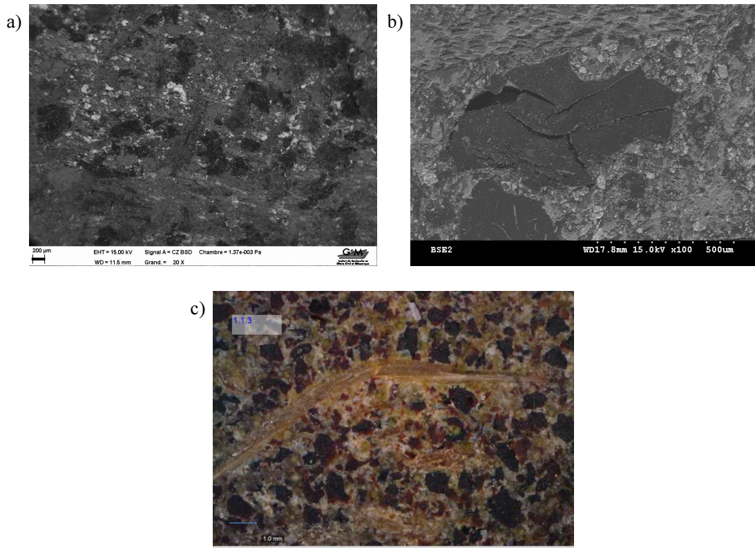
Fig. 2. Typical distribution of brass and rubber particles on surface of composite materials (a), shape of rubber particle (b), cluster of miscanthus fibers (c)
