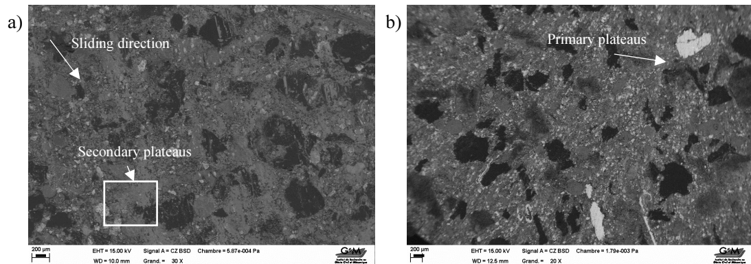
Fig. 3. Typical SEM micrographs showing general aspect of rubber and brass particles on rubbed surfaces at low braking energy (a and b)
