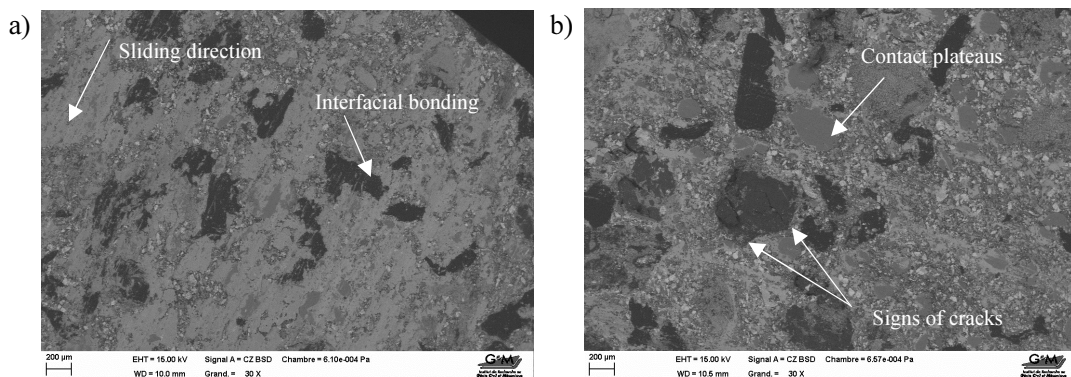
Fig. 5. Typical SEM micrographs showing general aspect of rubber and brass particles on rubbed surfaces at low and high braking energy (a and b)
