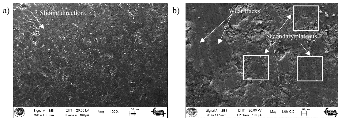
Fig. 4. Typical SEM micrographs showing general aspect of rubbed surface with presence of miscanthus fibers (a), detail of compacted friction layers at low braking energy (b)
