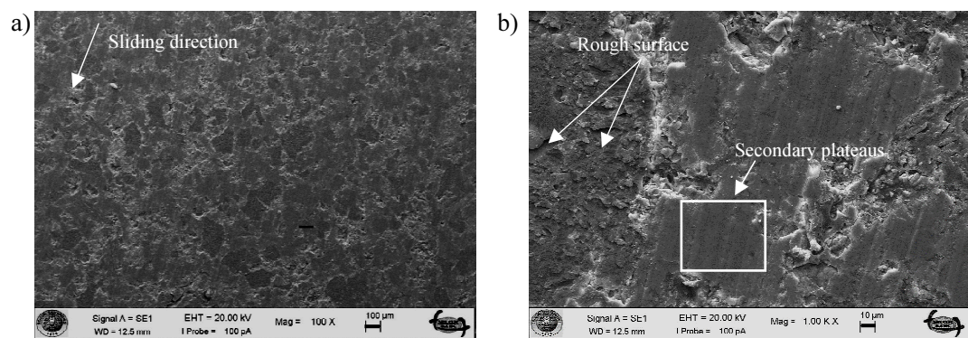
Fig. 6. Typical SEM micrographs showing general aspect of rubbed surface with presence of miscanthus fibers (a), detail of compacted friction layers at high braking energy (b)
