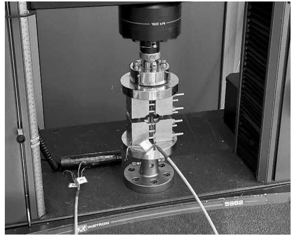
Fig. 7. Unidirectional specimen during compression test
