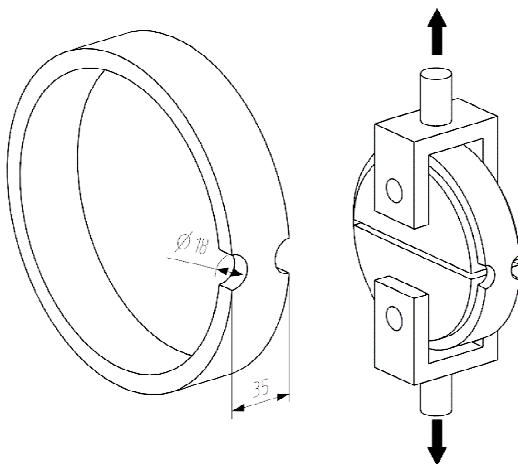
Fig. 10. Scheme of split disc test
