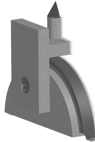
Fig. 11. FE model of split disc with fixture
