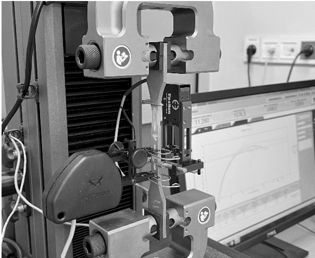
Fig. 9. PVC specimen during tensile test
