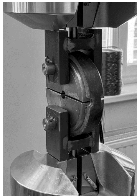
Fig. 15. Sample with fixture mounted on test machine
