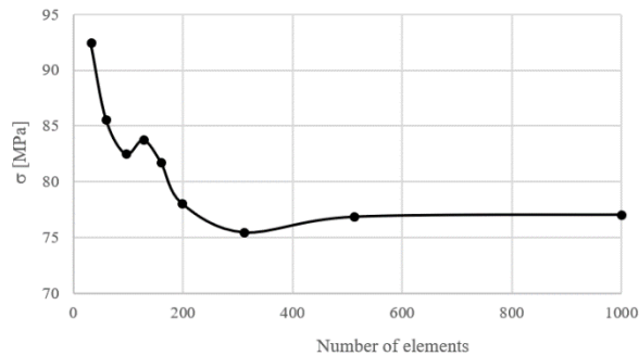
Fig. 13. Results of apparent tensile stress convergence study
