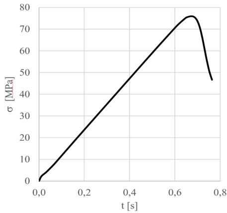
Fig. 12. Apparent tensile stress versus time diagram from FE simulation
